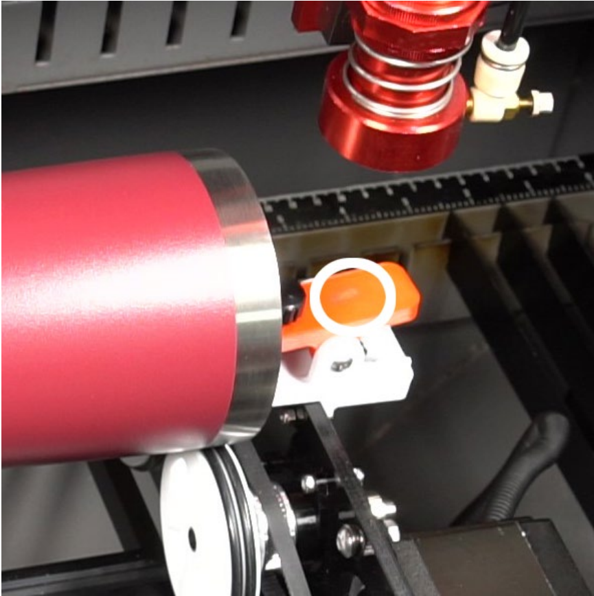
Figure 26. Center Alignment
