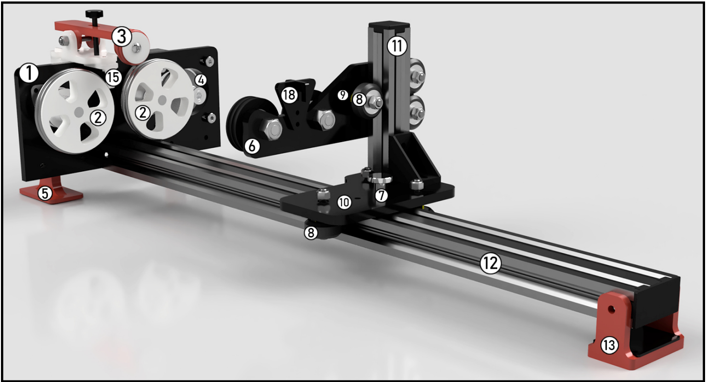
Figure 1. Front View
