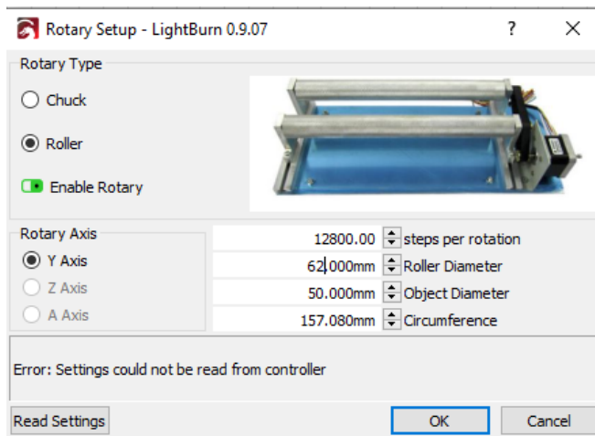
Figure 13. Lightburn Rotary Setup
