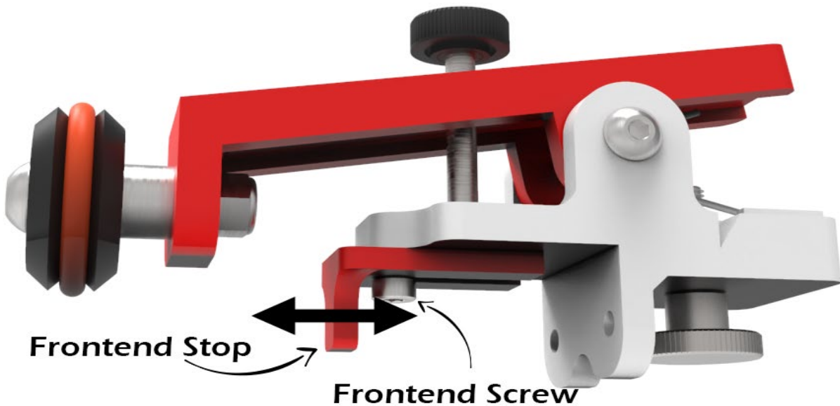
Figure 27. Front Endstop Adjustment
