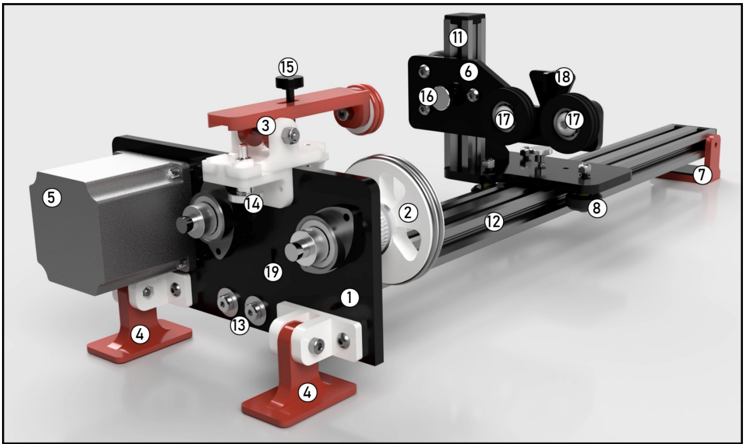
Figure 2. Back View
