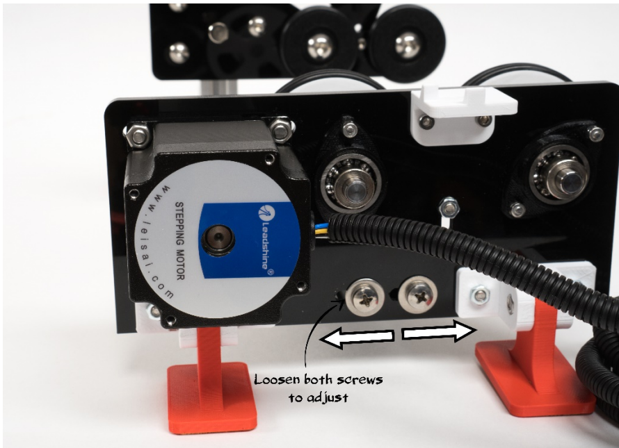
Figure 31. Headboard Screws
